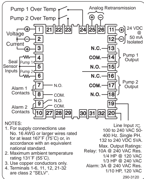
Figure 2 - Wiring
